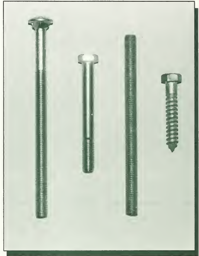
Figure 69—Fasteners (from left): carriage bolt, machine bolt, threaded rod, and lag screw.
